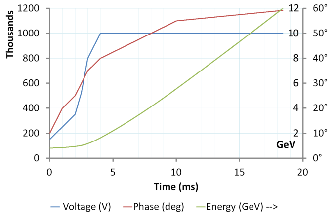
FIG. 15. RF acceleration program for the 12 GeV VFFAG.
