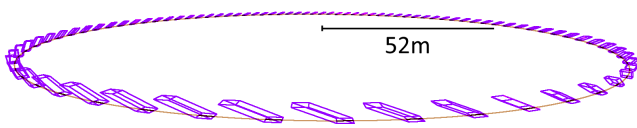
FIG. 8. Perspective view of the 12 GeV ring.
