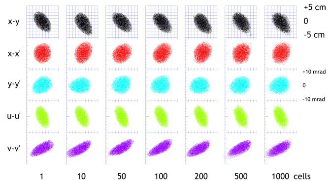
FIG. 11. Tracking through \sim 12 turns of the 12 GeV ring with matched beams (no space charge). Optics stable apart from signs of a 5 th order resonance in the (u, u') plane, since \mu_u \simeq 72^\circ
