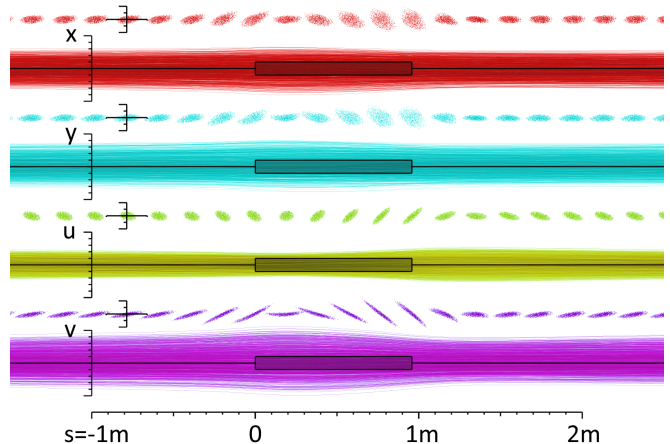
FIG. 10. Phase space and beam evolution through the 12 GeV ring cell at injection energy. Transverse scale is \pm 5 cm and x', y', u', v' ranges are \pm 20 mrad.
