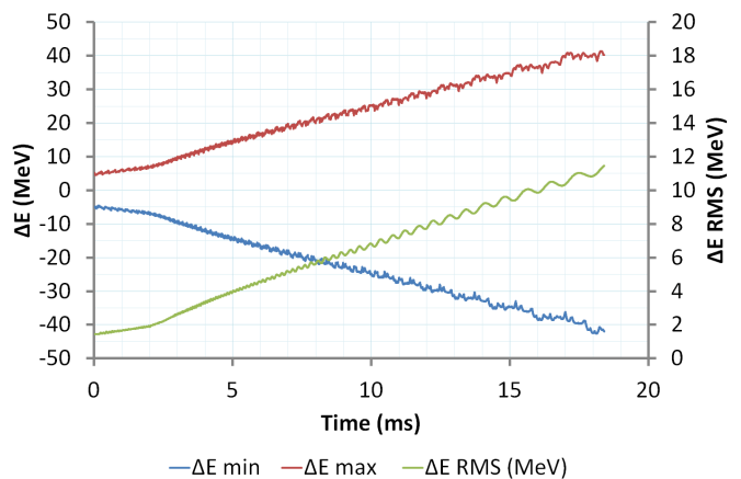
FIG. 18. Increase of bunch energy spread in the 12 GeV VFFAG simulation to \pm 41.1 MeV.
