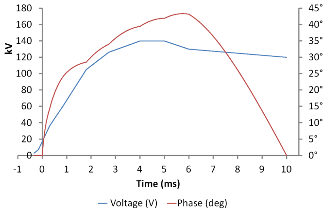
FIG. 13. ISIS first harmonic rf program.
