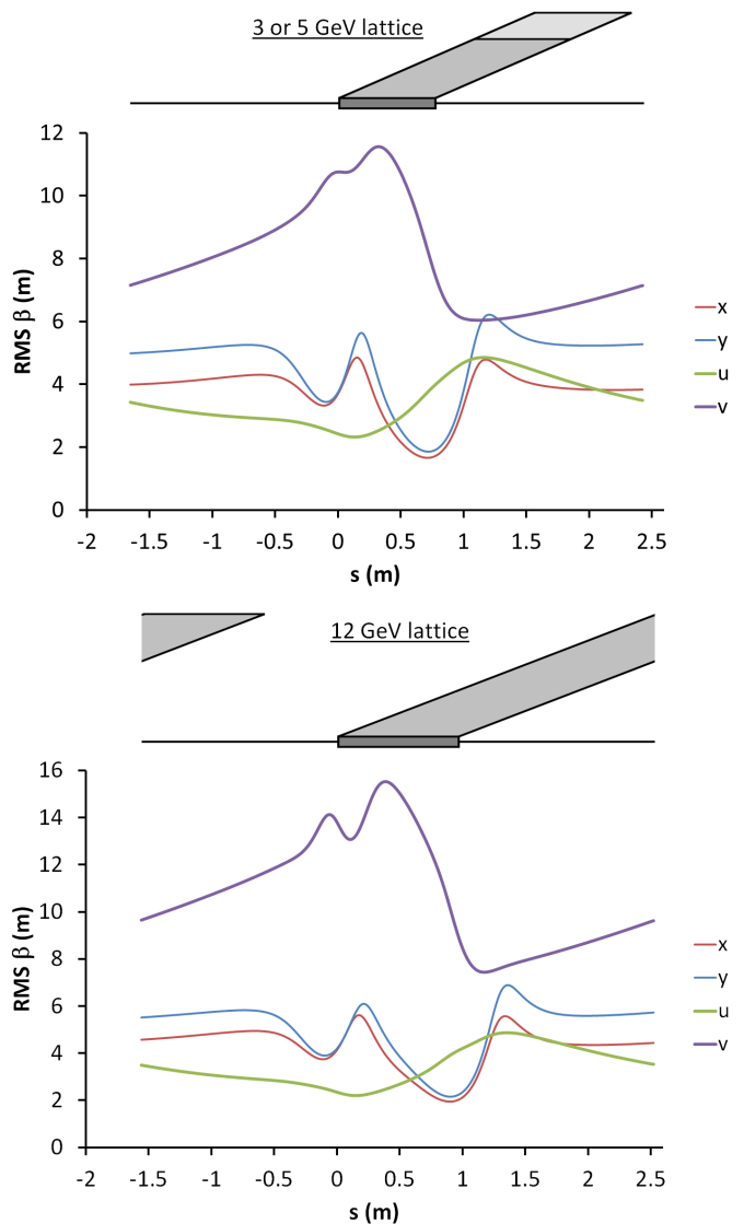
FIG. 9. RMS beta functions ( \beta_x^{\text{rms}} = \sigma_x^2 / \epsilon_x^{\text{rms}} ) of the beam distribution at injection in the two lattices, in non-skew and skew coordinates. In the schematic cell diagrams, magnet size is to scale in z and y .
