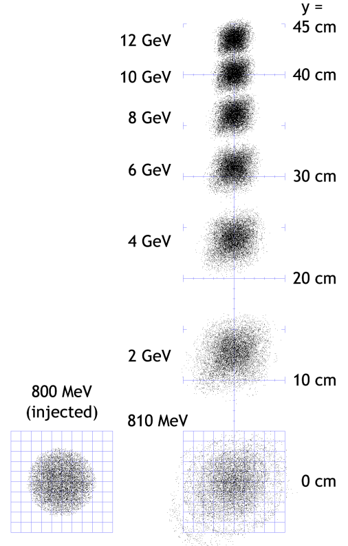
FIG. 1. Vertical movement of a proton beam accelerated in a scaling VFFAG with k = 5 \text{ m}^{-1} [3].
